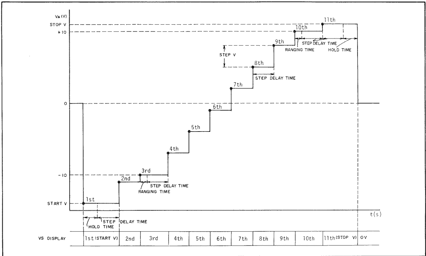
Figure 3-7 Relationship between Output Voltage and Display for \lrcorner (Single Staircase Wave).
