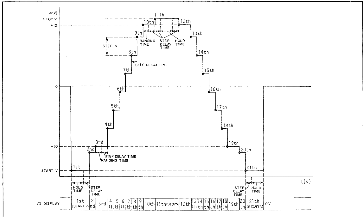
Figure 3-8. Relationship between Output Voltage and Display for \lrcorner (Double Staircase Wave).
