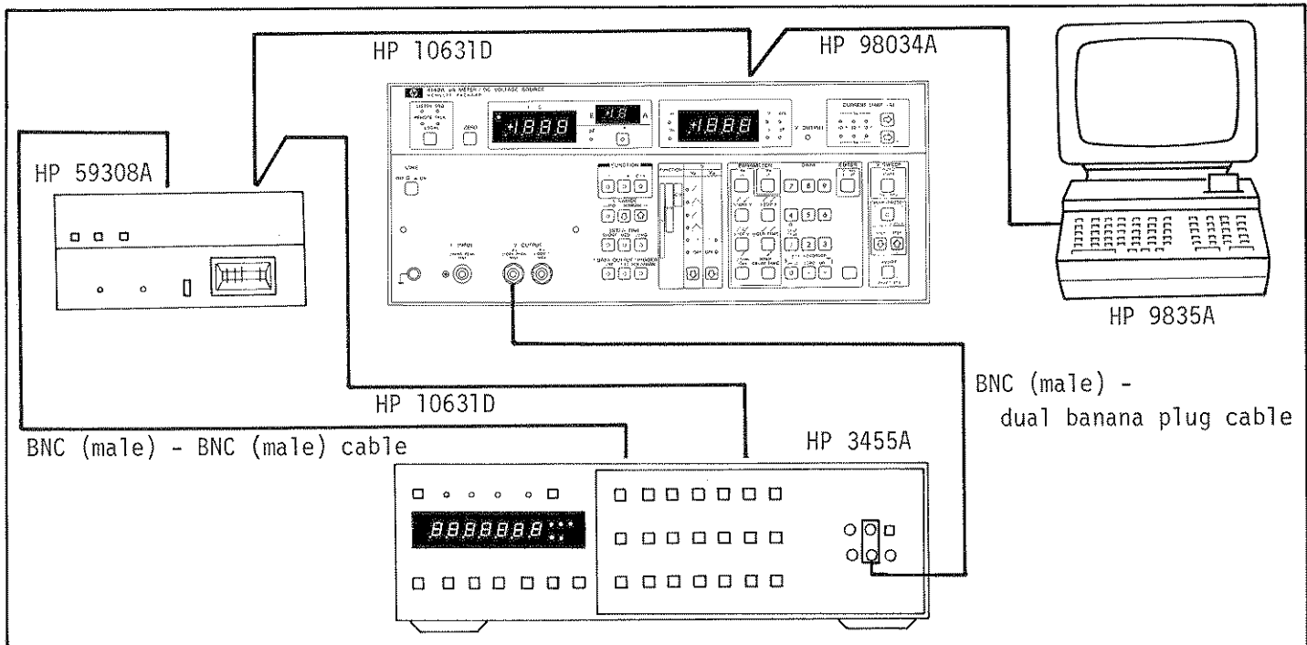
Figure 4-6. Ramp Rate Accuracy Test Setup.
