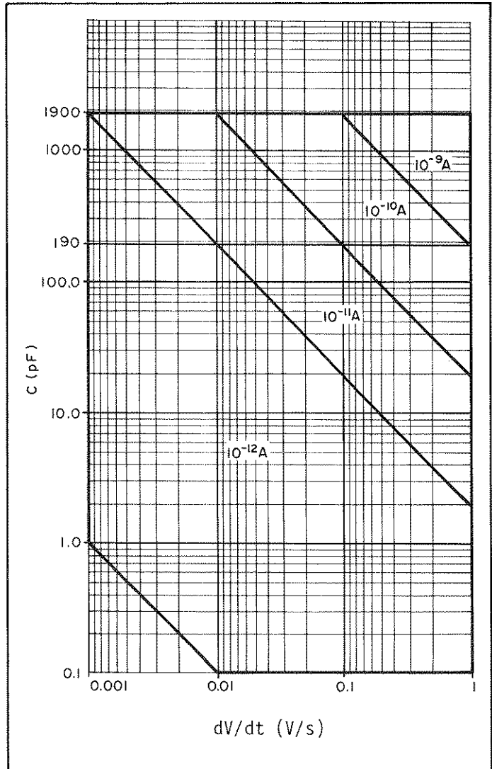
Figure 3-21. Suitable Current Measurement Ranges for C-V Measurements.
