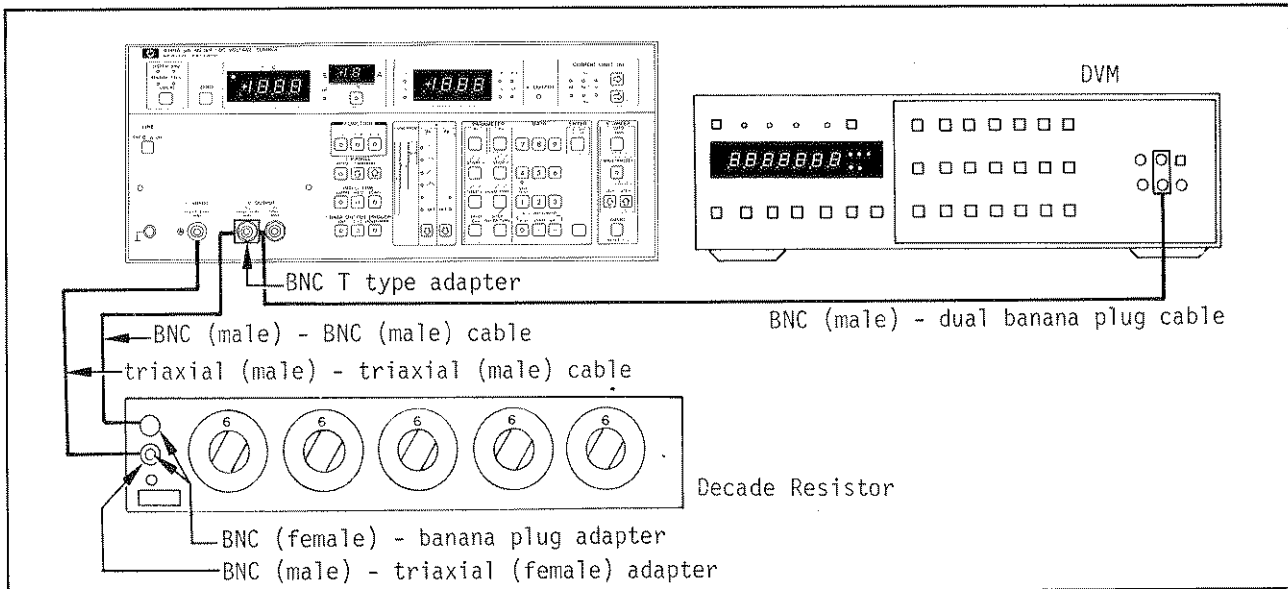
Figure 4-2. Current Measurement Accuracy Test Setup ( 10^{-2}A \sim 10^{-7}A Ranges).
