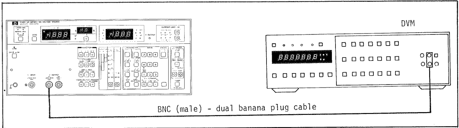
Figure 4-5. Ramp Wave Start Voltage Accuracy Test Setup.
