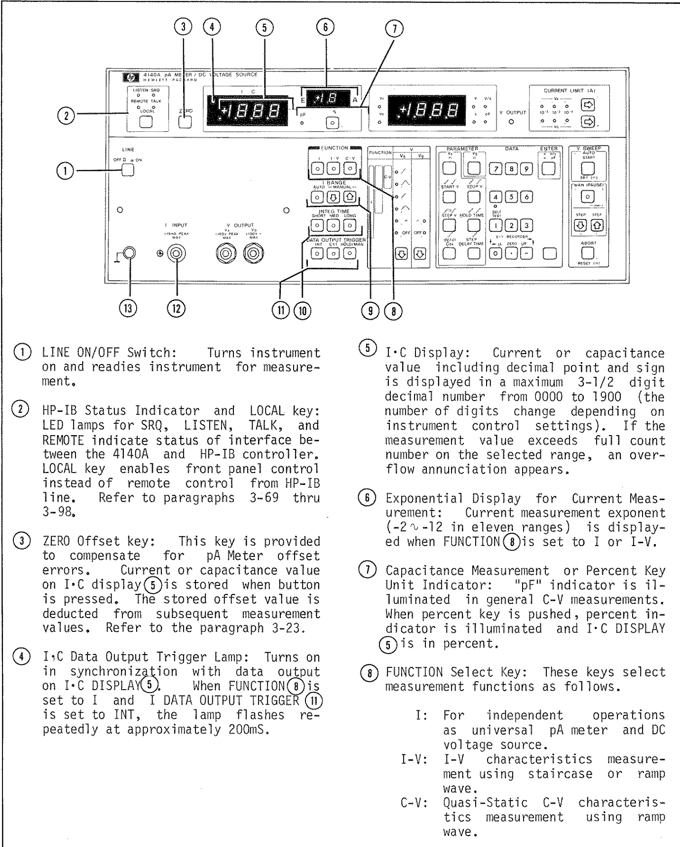
Figure 3-1. Front Panel Features (sheet 1 of 5).
