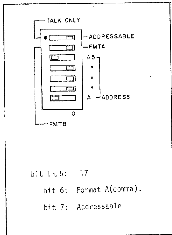
Figure 3-25. HP-IB Control Switch.
