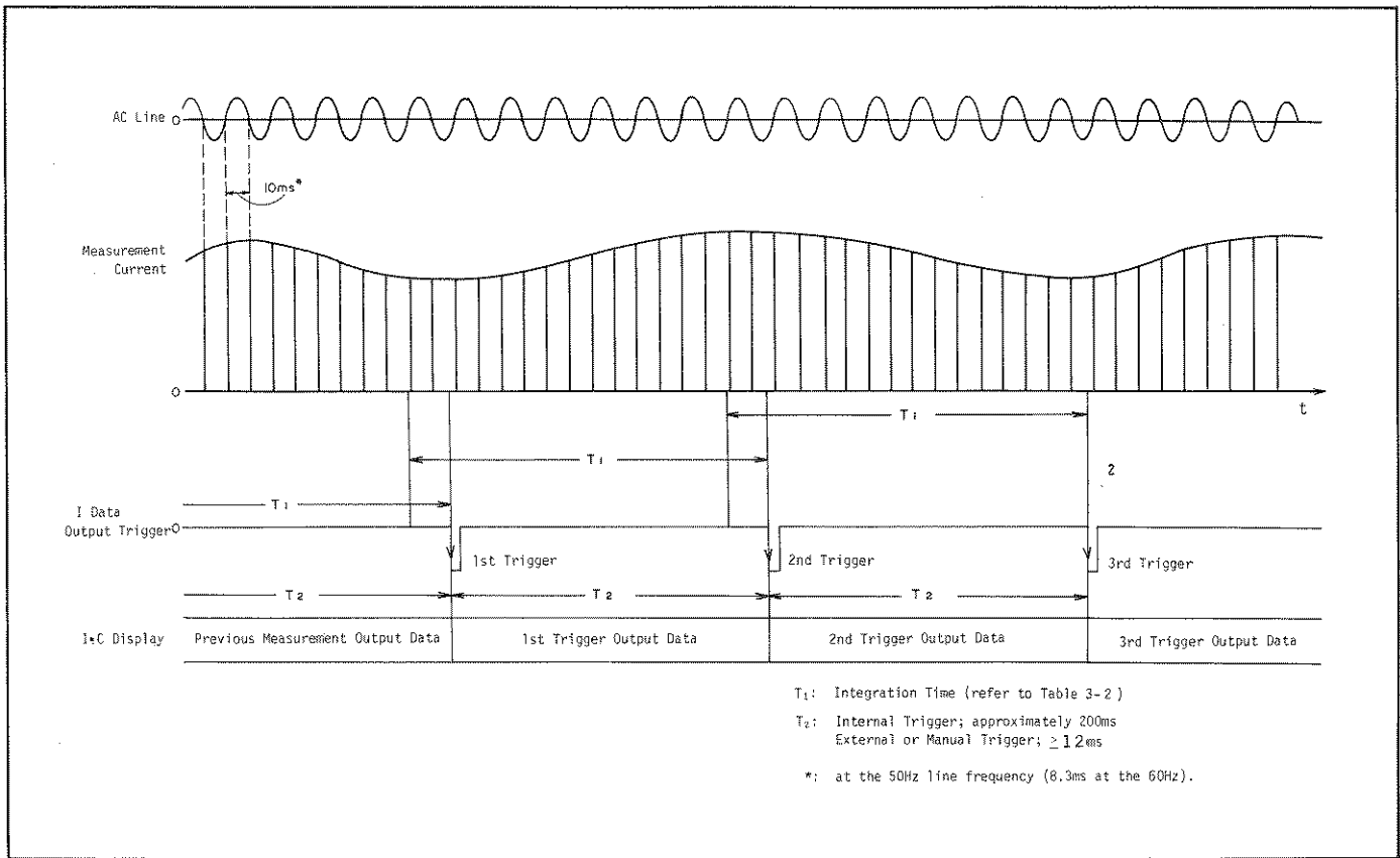
Figure 3-5. Integration Time and Data Output (When FUNCTION is Set to I).
