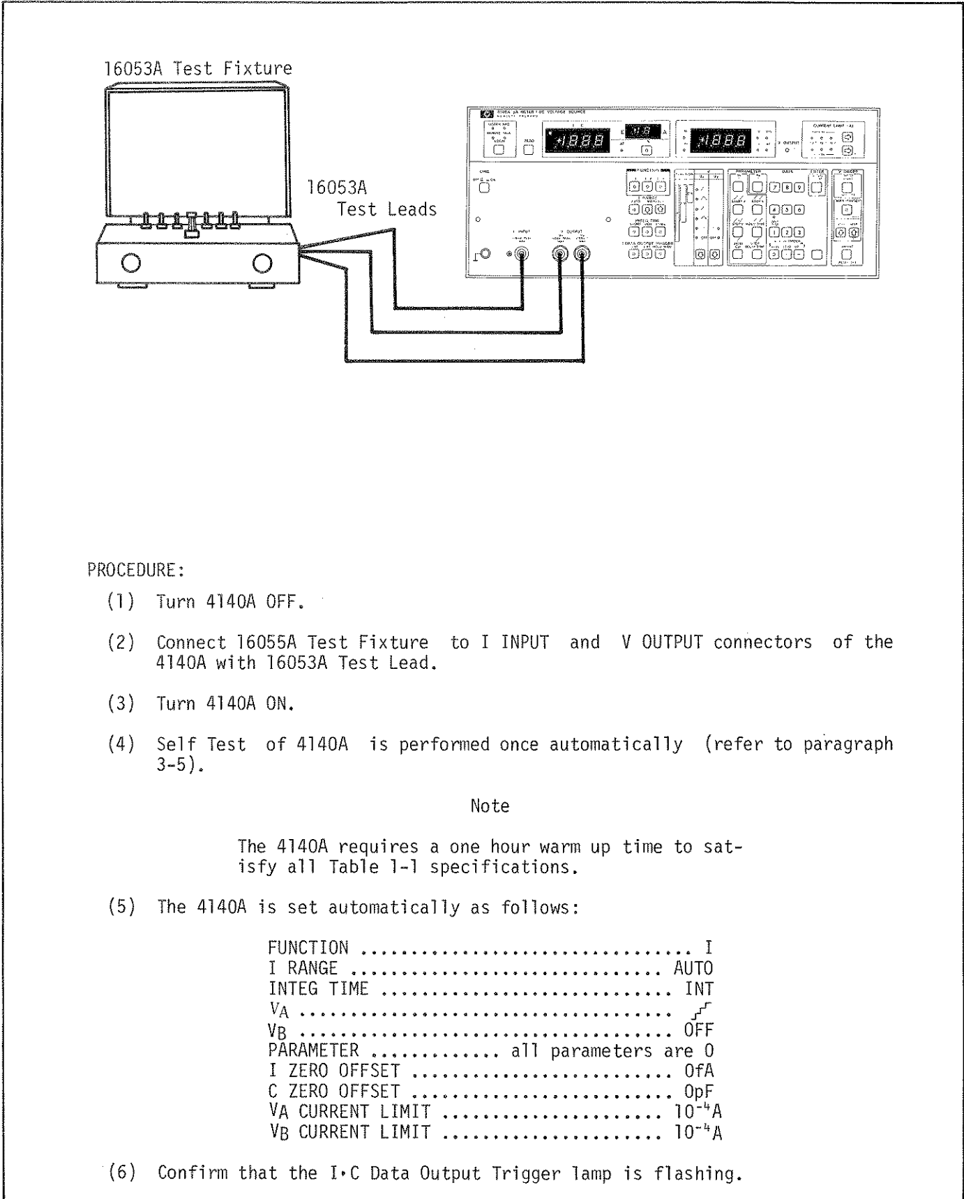
Figure 3-23. C-V Function Operating Instructions (sheet 1 of 3).
