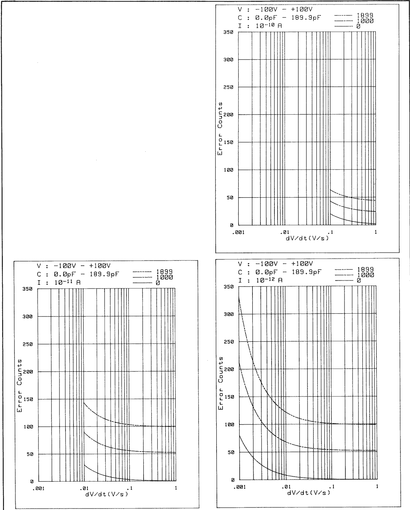
Figure 3-22. C-V Measurement Accuracy (Sheet 3 of 4).
