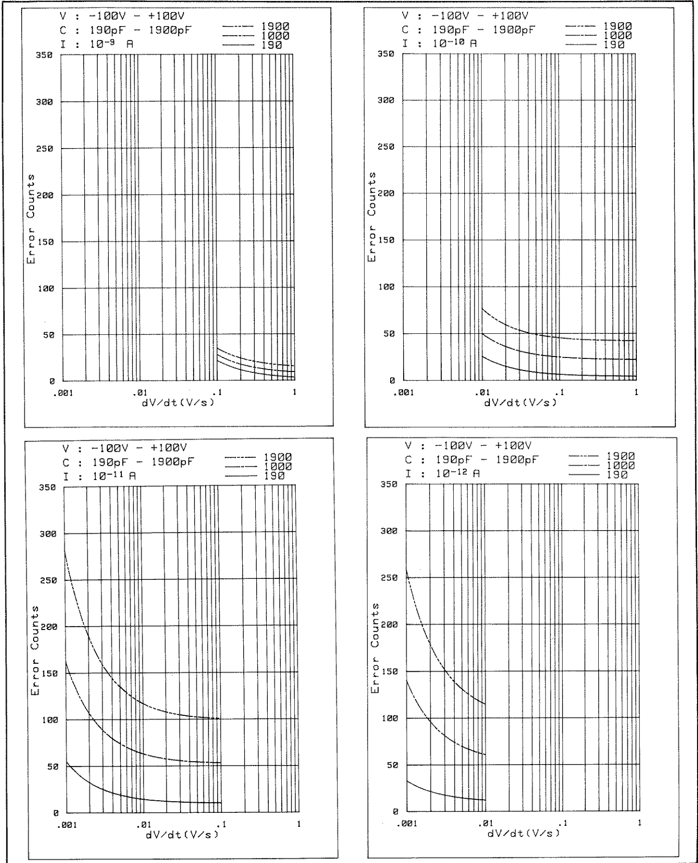
Figure 3-22. C-V Measurement Accuracy (Sheet 4 of 4).
