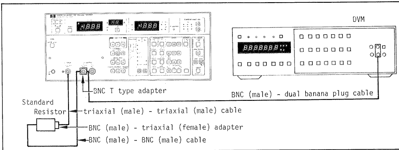
Figure 4-3. Current Accuracy Test Setup ( 10^{-8}A \sim 10^{-12}A Ranges).
