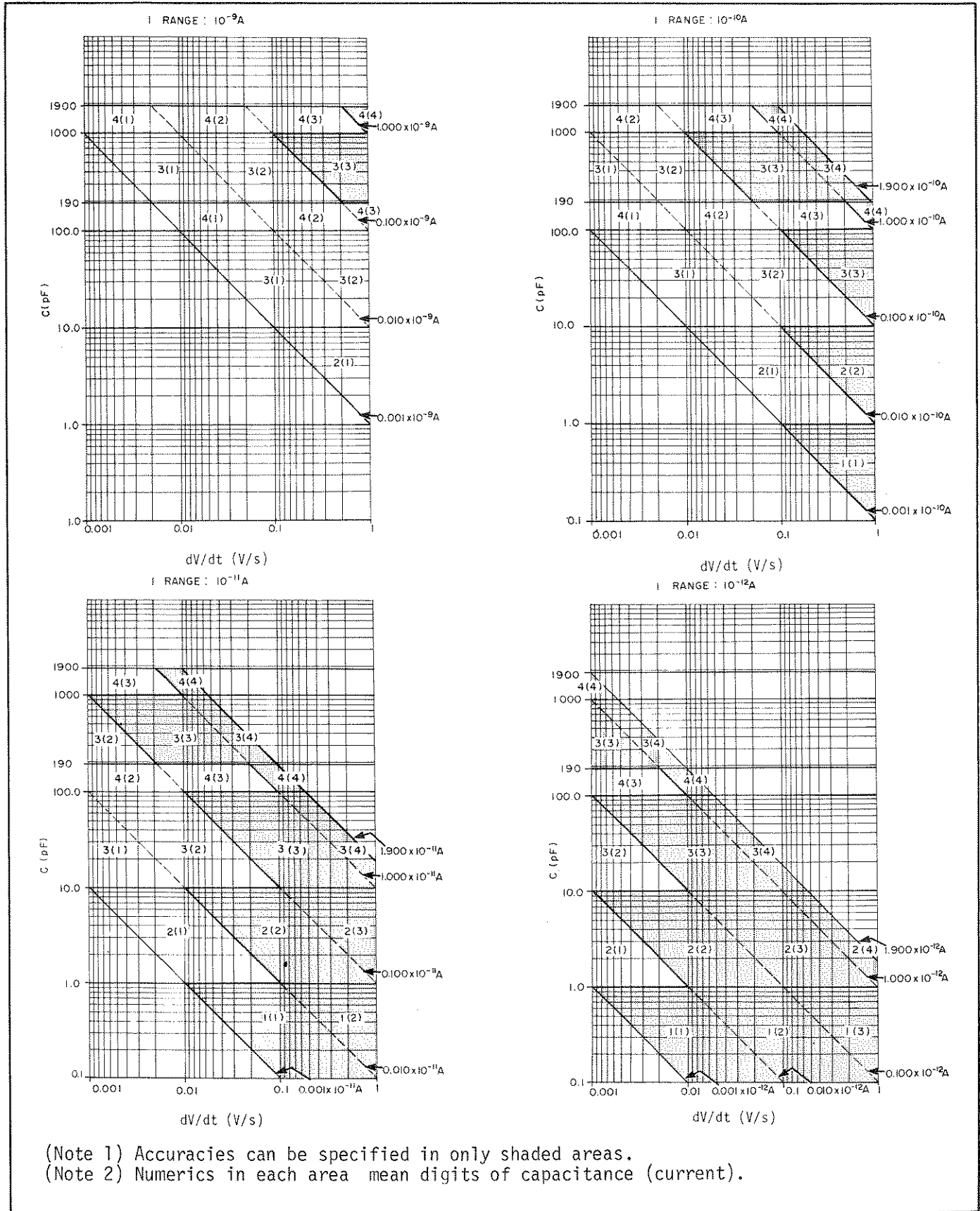
Figure 3-20. Relationship between Calculated Capacitance Value and Current Measurement Range.
